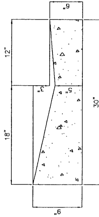
DETAIL "A" TYPICAL VALLEY GUTTER
